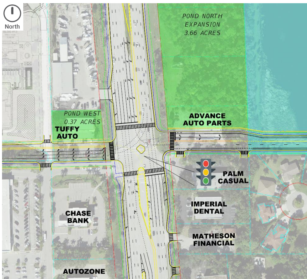
Figure 1-8: US 41/Center of Bonita Springs “Thru-Cut” Intersection
