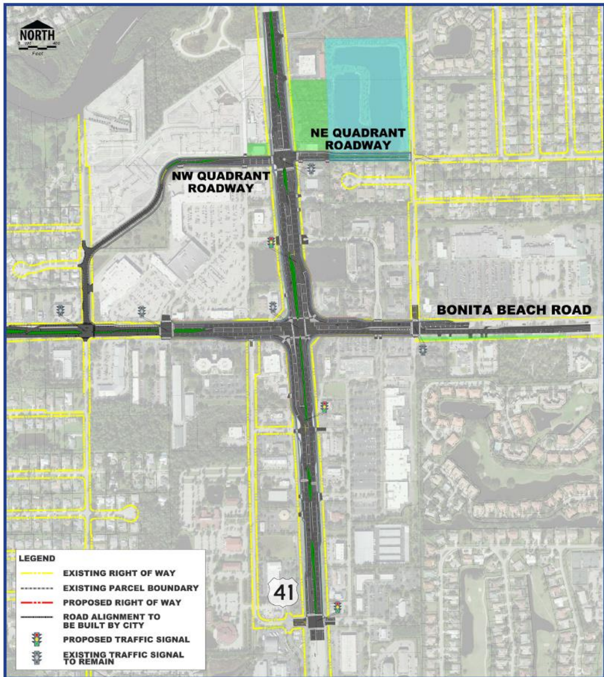
Figure 1-6: Preferred Alternative Improvements in Study Area
