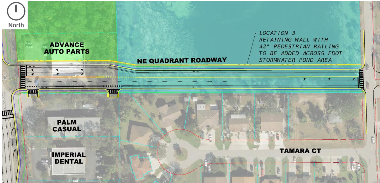
Figure 1-10: Northeast Quadrant Roadway – East Leg at US 41
