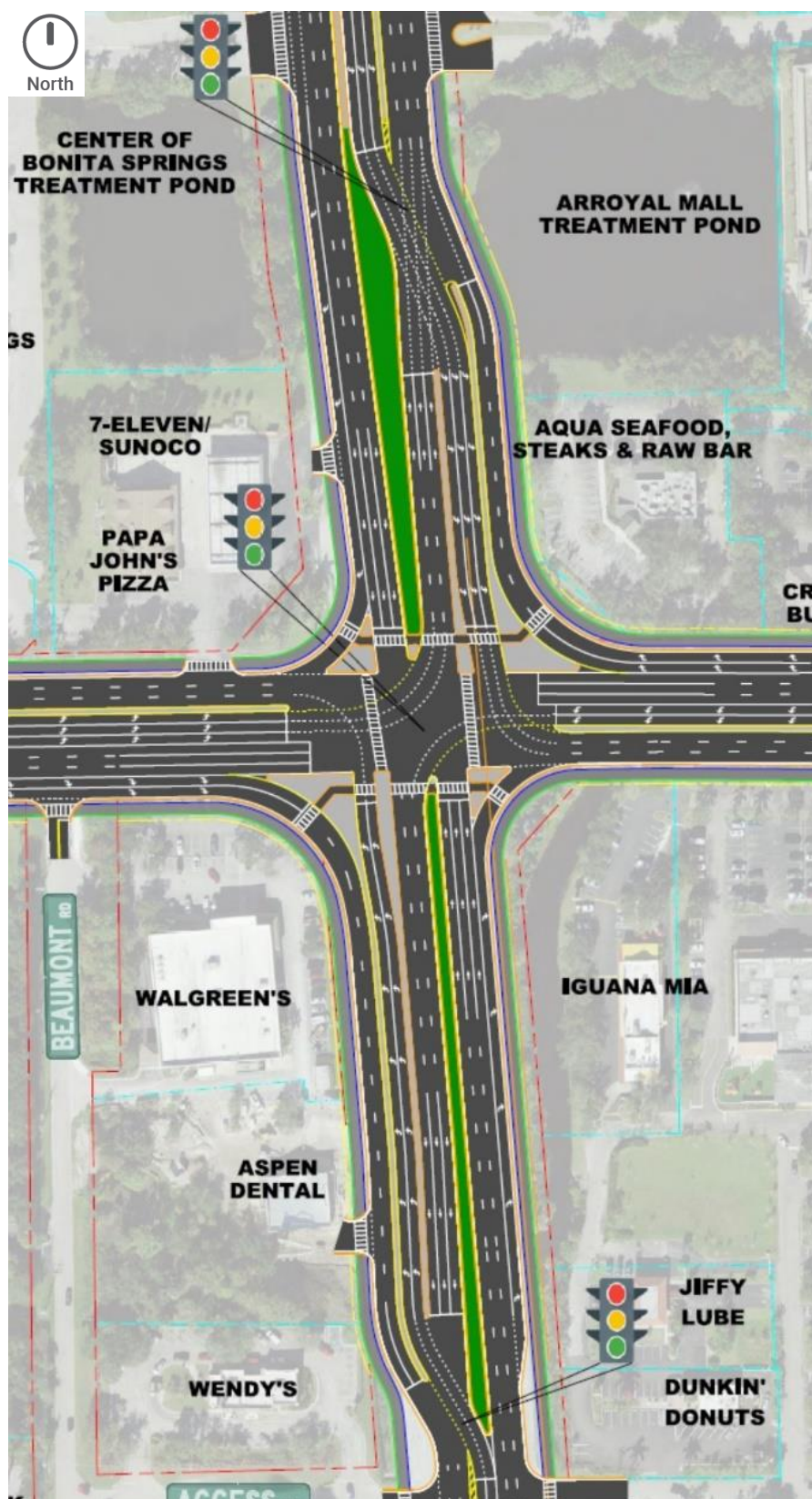
Figure 1-7: Partial Displaced Left Turn Detail
