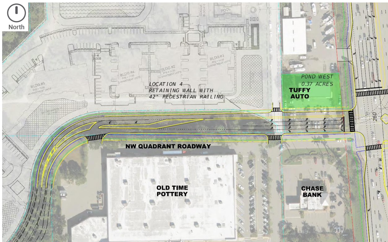
Figure 1-9: Northwest Quadrant Roadway – West Leg at US 41
